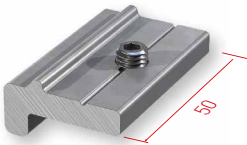
F85-456 Kama kilidi Pressure plate restrainer
